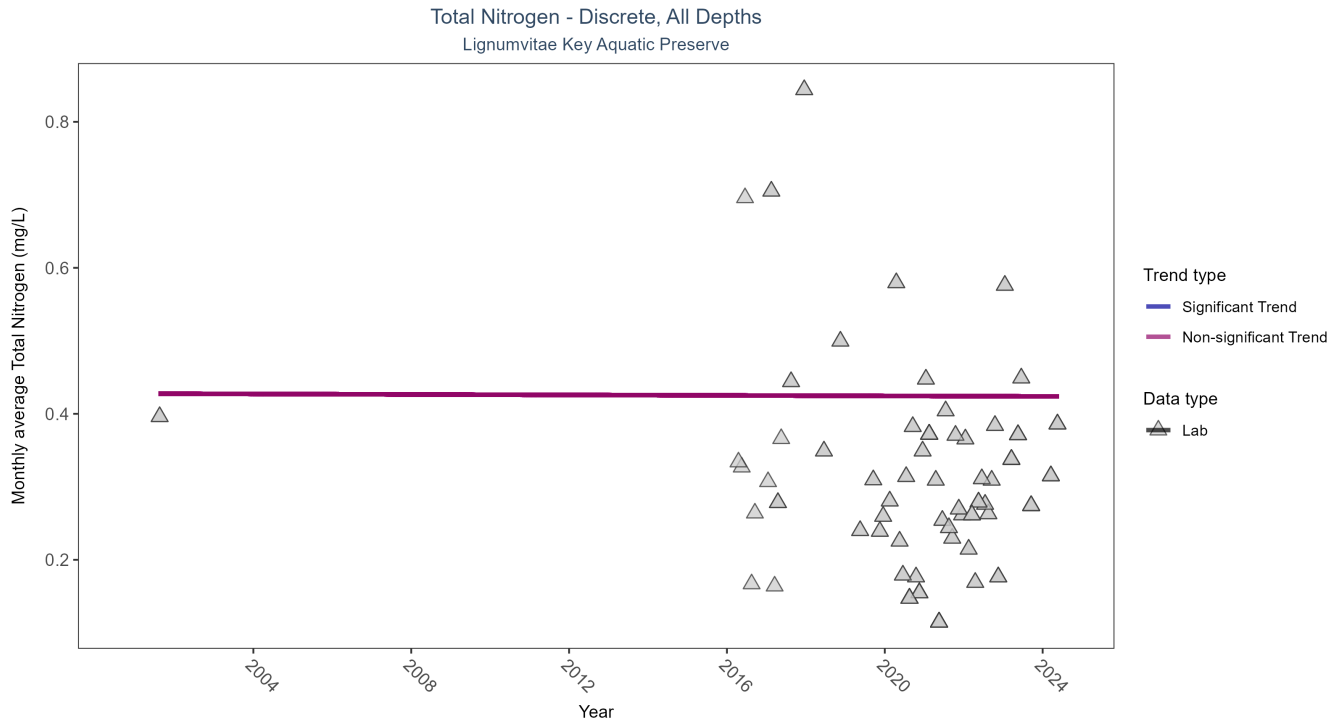
Figure 9: Seasonal Kendall-Tau Results for Total Nitrogen - Discrete
