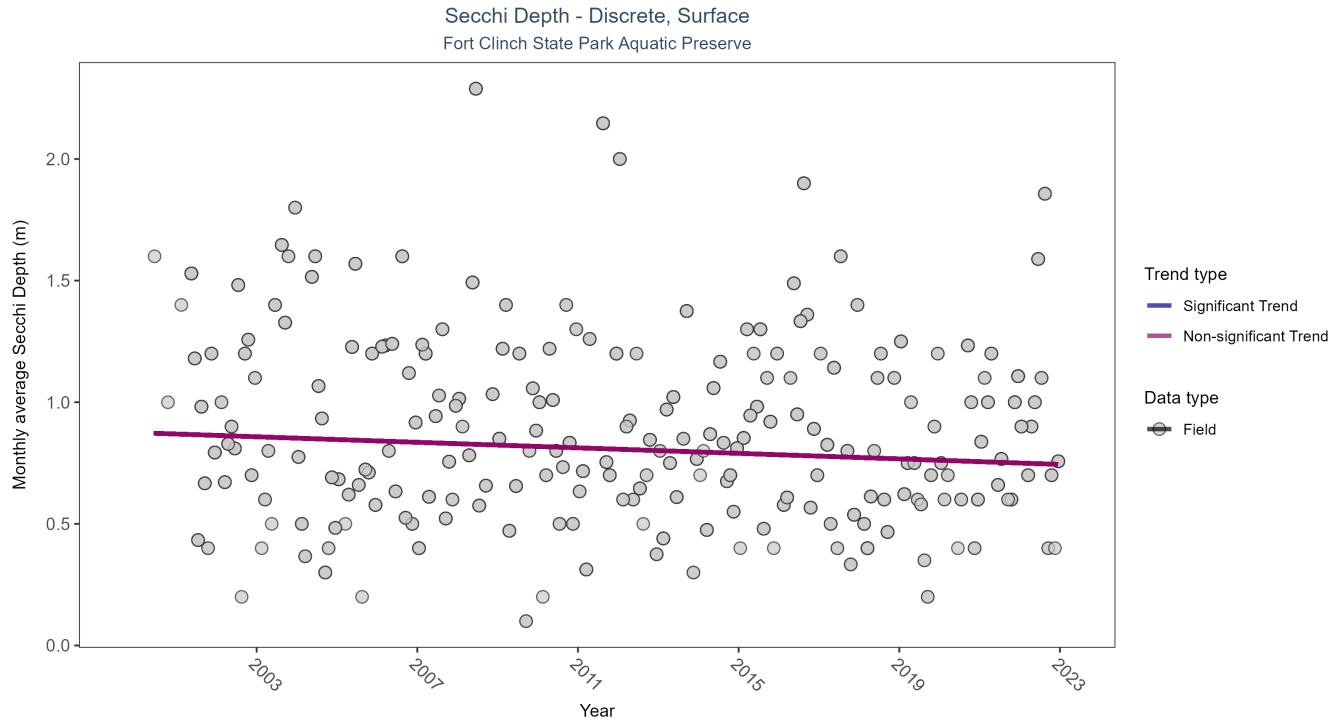
Figure 7: Seasonal Kendall-Tau Results for Secchi Depth - Discrete
