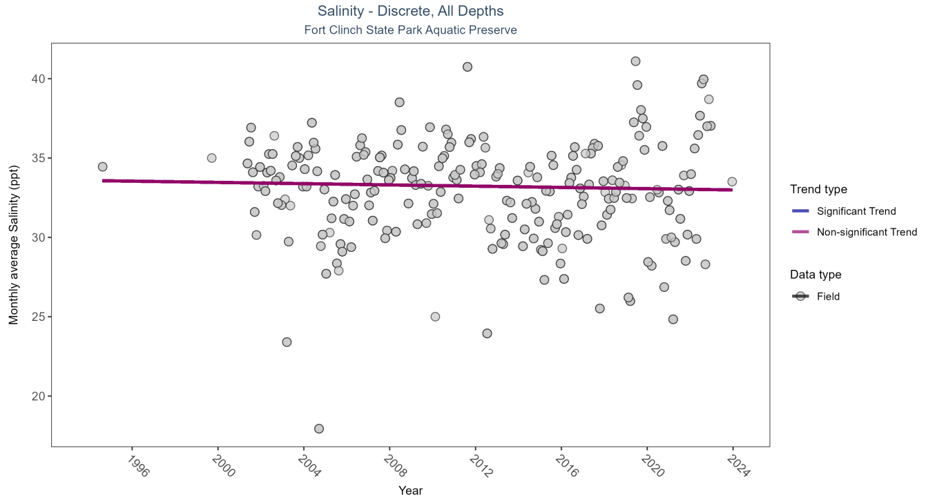
Figure 5: Seasonal Kendall-Tau Results for Salinity - Discrete
