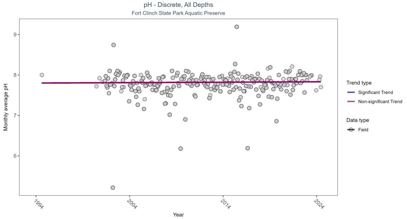
Figure 3: Seasonal Kendall-Tau Results for pH - Discrete
